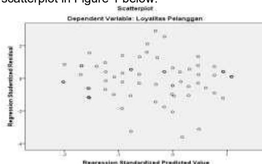
Figure 2. Heteroscedasticity Test
