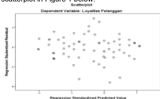
Figure 2. Heteroscedasticity Test
